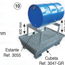
Cubeta Ref. 3047-GR
